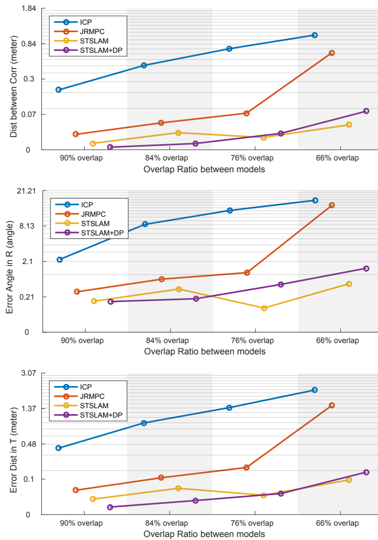
Figure 1. Registration accuracy of our method (STSLAM) compared to (ICP) [1] and joint registration (JRMP) [2] measured by average closest point distance (Top), rotation angle error (middle), and translation error (bottom).
