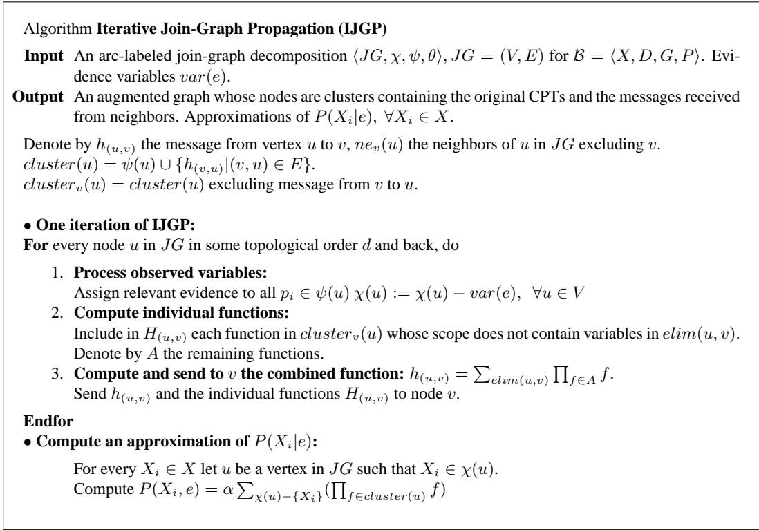
Figure 13: Algorithm Iterative Join-Graph Propagation (IJGP).
