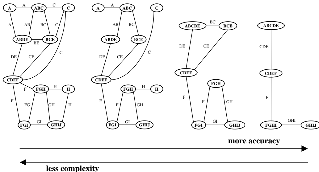
Figure 19: Join-graphs.
