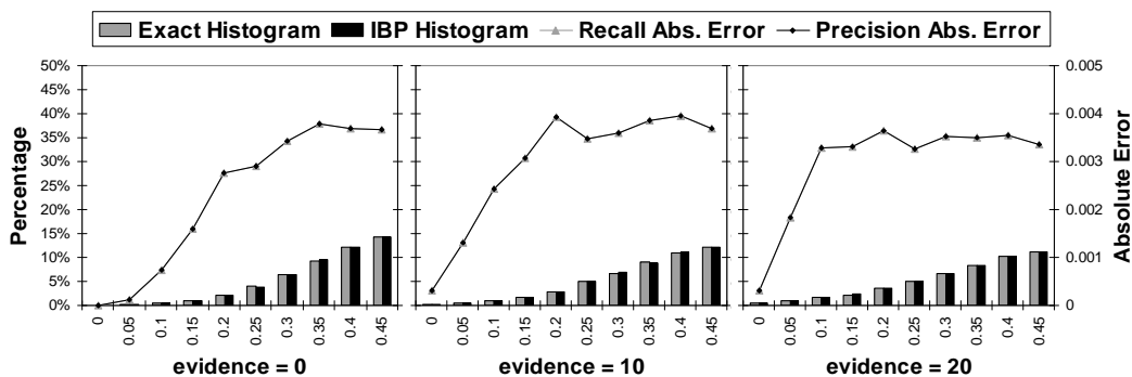
Figure 22: 10x10 grids, 100 instances, w^*=15 .
