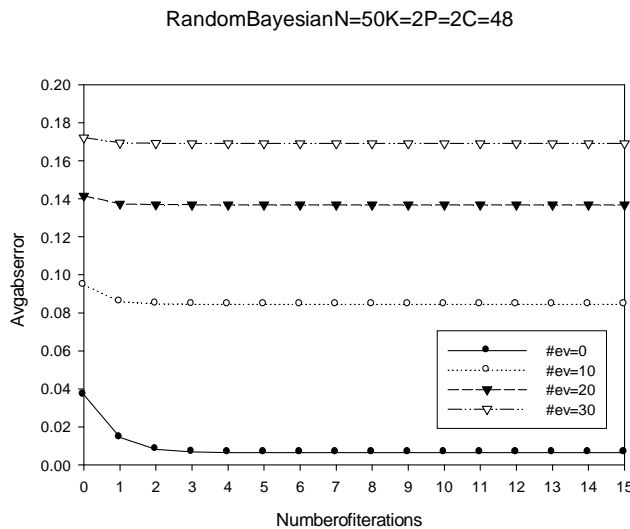
Figure 6: Convergence of IBP (50 variables, evidence from 0-30 variables).
