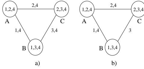
Figure 12: An edge-labeled decomposition.
