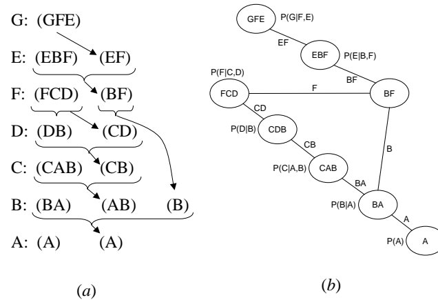
Figure 18: Join-graph decompositions.
