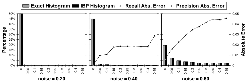
Figure 21: Coding, N=200, 1000 instances, w^*=15 .
