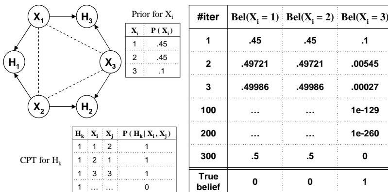
Figure 20: Example of a finite precision problem.
