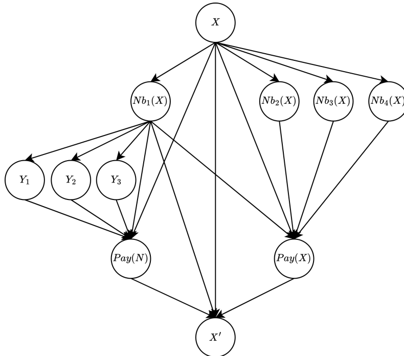
Figure S2: Example (simplified) Bayesian network corresponding to an 8 node SD-BNA for an evolutionary game
