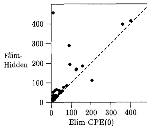
Figure 12: 50 test instances of the insurance network with query parameters \langle 15, 5 \rangle
