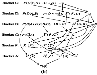
Figure 3: Trace of Elim-CPE (a) no observation (b) with observation
