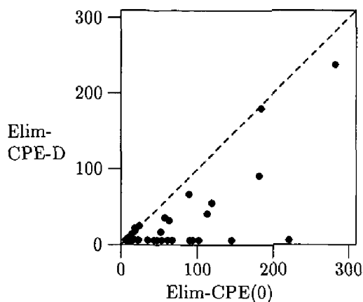
Figure 9: 48 test instances with network parameters \langle 80, 4, 0.75 \rangle and query parameters \langle 0, 10 \rangle
