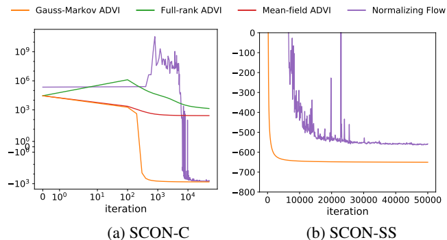
Figure 2. Trace plots of negative ELBO loss, estimated from 100 samples every 100 iterations. MF-ADVI converges to suboptimal loss, while FR-ADVI fails to converge within 50,000 iterations. In (b), we highlight that normalizing flow converges to worse loss than GM-ADVI and is substantially more noisy.
