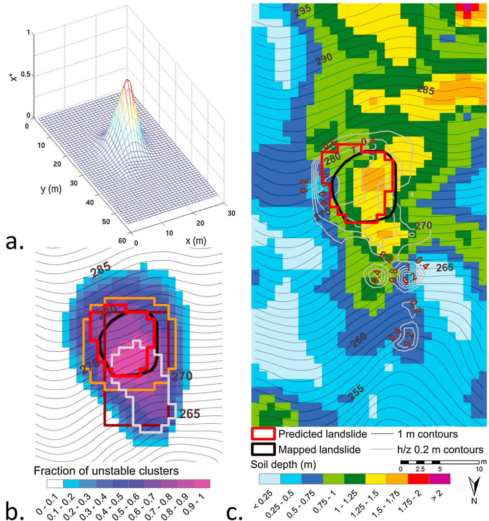
Figure 7. Application of the model to the CB-1 experimental catchment. (a) The first eigenvector \mathbf{x}^* , which corresponds to the smallest eigenvalue of the linear system defined by equation (12). (b) The outlines of the search algorithm predictions with the minimum FS (red), the maximum FS below unity (gray); those from an exhaustive rectangular search (dark brown), and from an exhaustive elliptical search (light brown); the observed CB-1 landslide (black). The landslides are overlaid on a map showing 1 m elevation contours (thin black lines) and the fraction of the 475 predicted landslide shapes that include each grid cell. (c) The outlines of the search algorithm prediction with the minimum FS (red) and of the observed CB-1 landslide (black). The landslides are overlaid on a map showing 1 m elevation contours, 0.2 m/m saturation ratio ( h/z ) contours, and the soil depth grid. Data from Montgomery et al. [2009] .
